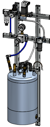
55 00 0300.003 VBG-MDJ10L-01-1Z-2V-024DC-VS
